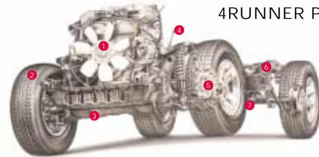
A strong coil-spring, double-wishbone front suspension provides lots of wheel travel – a major benefit to rock crawlers and highway commuters alike. Complementing this design is a solid-axle 4-link/coil spring rear suspension.
